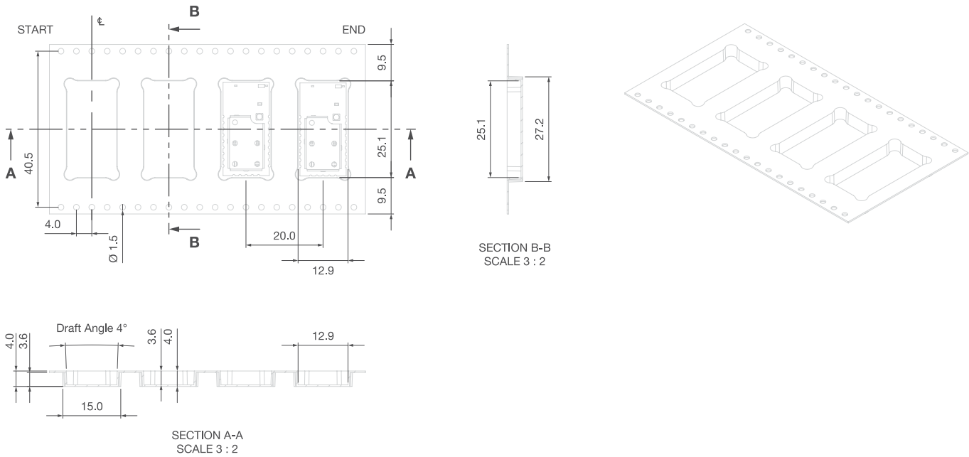
FIGURE 9.1-1 TAPE&REEL PACKAGING
