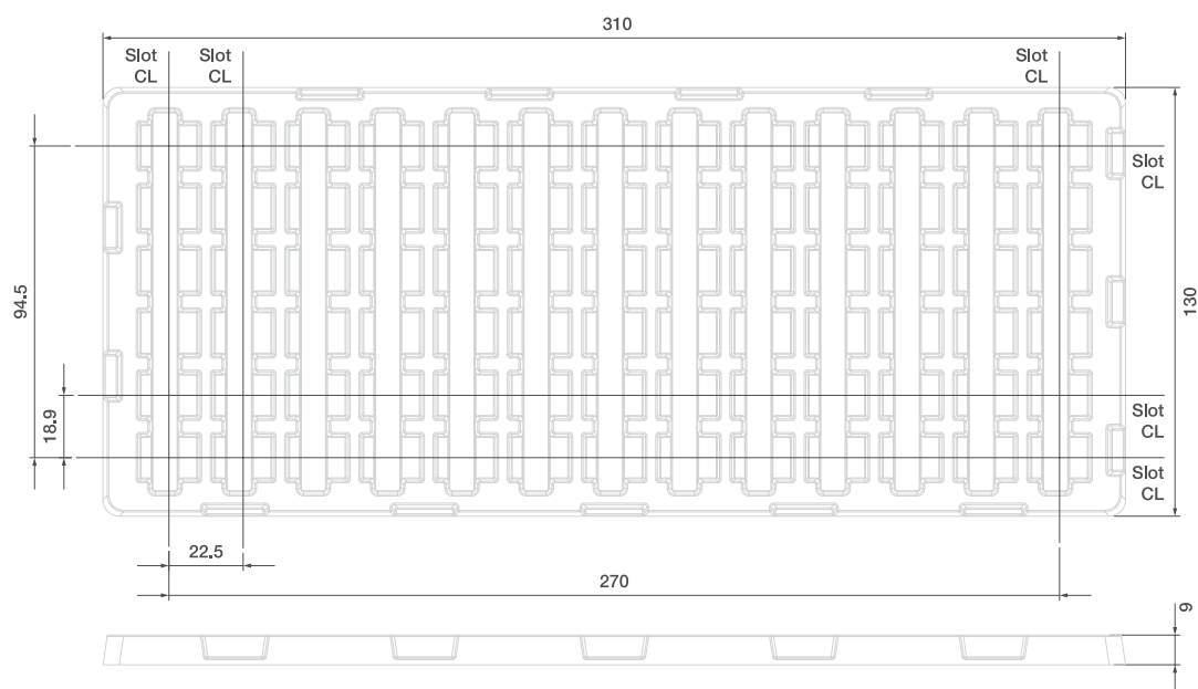
FIGURE 9-2. RED-BEAN-C TRAY
