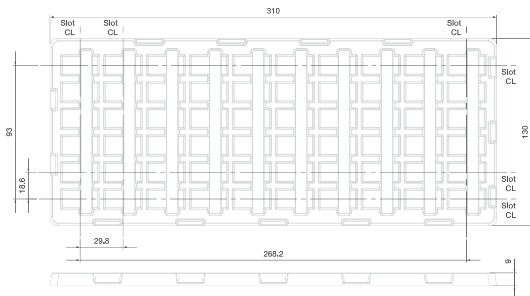
FIGURE 9-1. RED-BEAN-A TRAY
